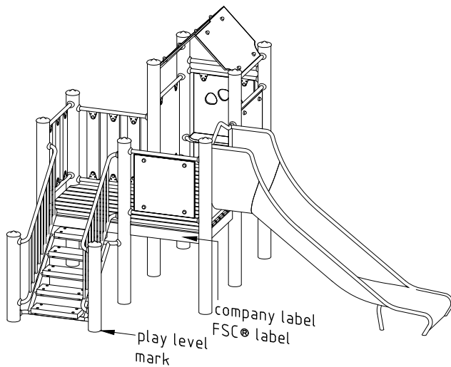
detail of play level mark
